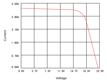
Module IV Graph 50W
